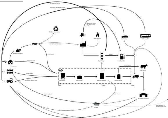
A new combined waste & wastewater recycling strategy for Truford Park, Manchester
